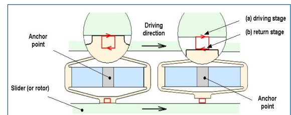
RPMHPP motor - Schematic view.
