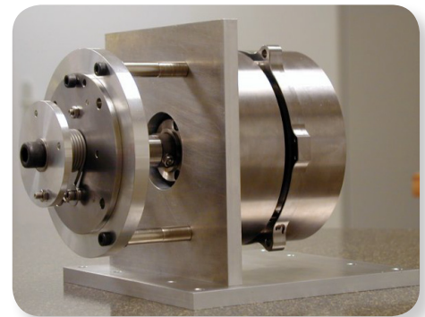
RPMHPP motor.
